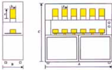
GRADIGENT KILN, Model GR / 98 and GR / 98 S
