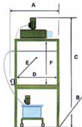
SPRAY CABIN Mod. F / 80 With Water Veil
